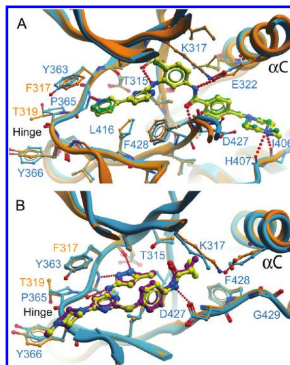
Figure 2. Comparison of ABL2:imatinib and ABL2:1 with ABL1:imatinib and ABL1:1. (A) Imatinib bound in the active sites of ABL1 and ABL2. The structure of the active site of ABL1 with imatinib bound (blue) (PDB code 1IEP) 22 is shown superimposed on ABL2:imatinib (orange), showing that the inhibitor molecules bind in the same conformation in both structures. Imatinib is shown in yellow for ABL2 and green for ABL1. (B) 1 bound in the active sites of ABL1 and ABL2. The structure of the active site of ABL1 with 1 bound (PDB code 2F4J) 24 is shown superimposed on ABL2:1. Coloring is as for (A) except that 1 is in yellow for ABL2 and purple for ABL1.
